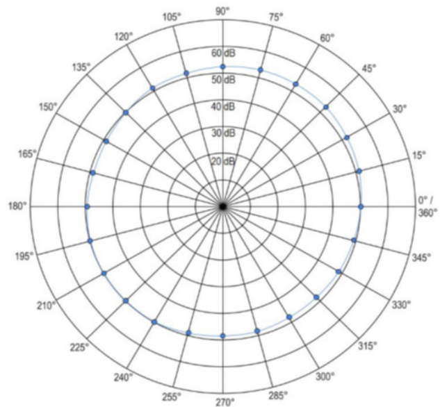
Radiation Pattern
